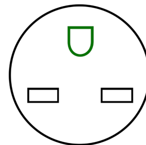
Plug Configuration NEMA 6-15
